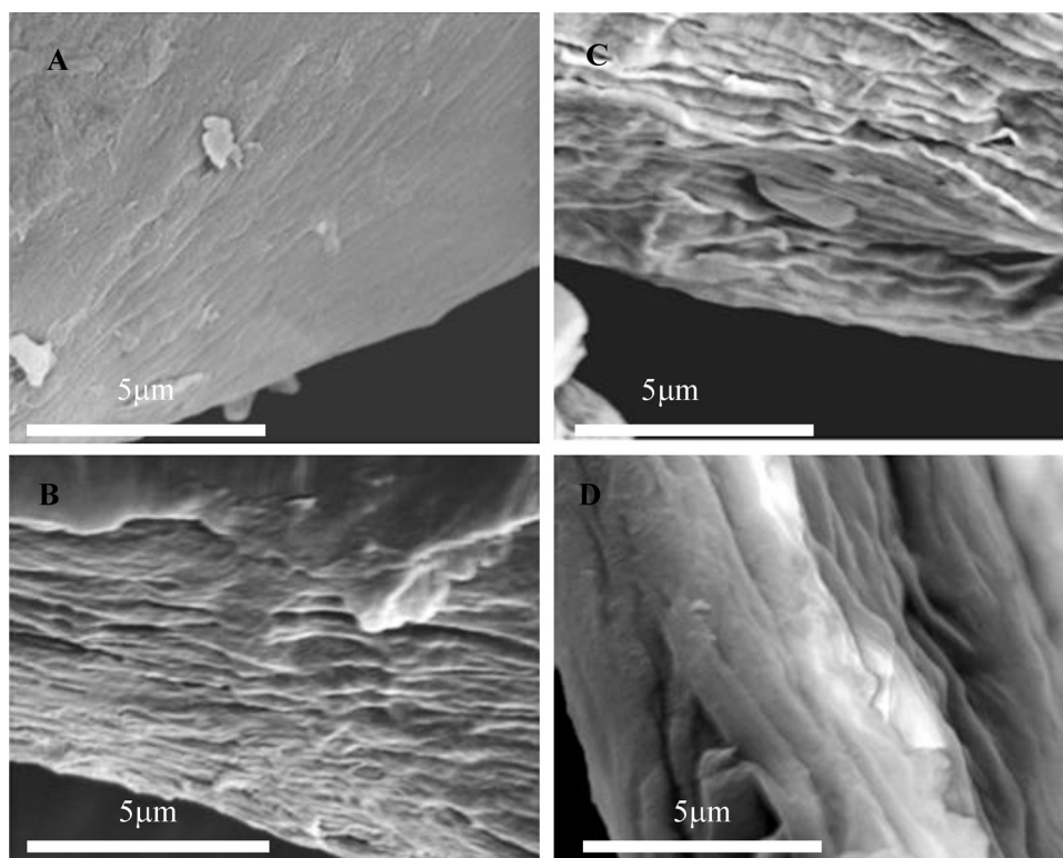
Fig. 8. SEM micrographs of (A) raw cellulose and solid samples after hydrolysis, (B) cellulose pretreated with 3 wt.% of sulfuric acid after 28 h of hydrolysis in oven, (C) cellulose pretreated with 6 wt.% of sulfuric acid after 28 h of hydrolysis in oven and (D) cellulose pretreated with 6 wt.% of oxalic acid after 6 h of hydrolysis in microwave.
