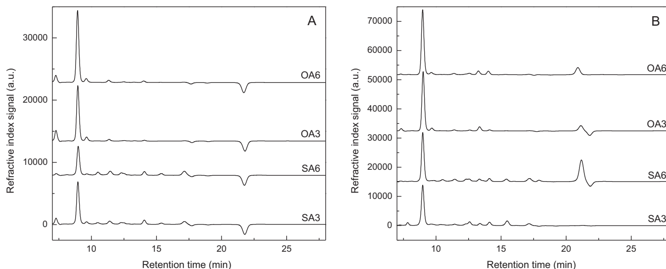
Fig. 1. HPLC chromatograms of selected liquid samples after hydrolysis in (A) oven and (B) microwave.
