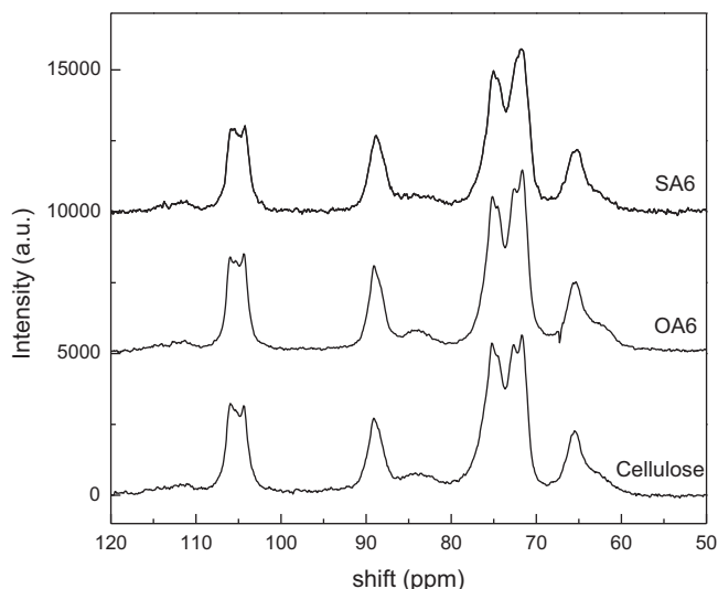
Fig. 7. NMR spectra of selected cellulose samples.
