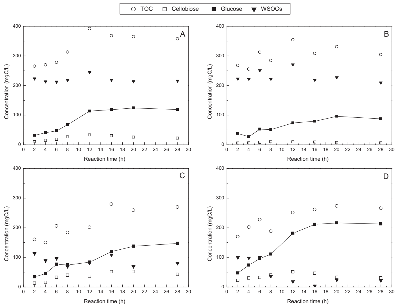
Fig. 2. Changes in aqueous product concentration (mg/L) versus reaction time during cellulose hydrolysis in a conventional hydrothermal treatment (oven) at 393 K. Cellulose samples pretreated with (A) 3 wt.% of sulfuric acid (SA3), (B) 6 wt.% of sulfuric acid (SA6), (C) 3 wt.% of oxalic acid (OA3) and D) 6 wt.% of oxalic acid (OA6).
