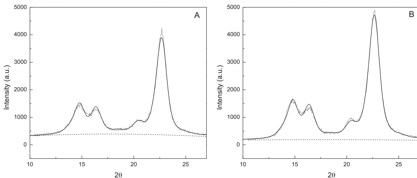
Fig. 6. XRD—Calculated and observed X-ray diffractograms for samples AS6 and AO6 after 28 h of hydrolysis in a conventional oven showing the peak position for the amorphous part.
