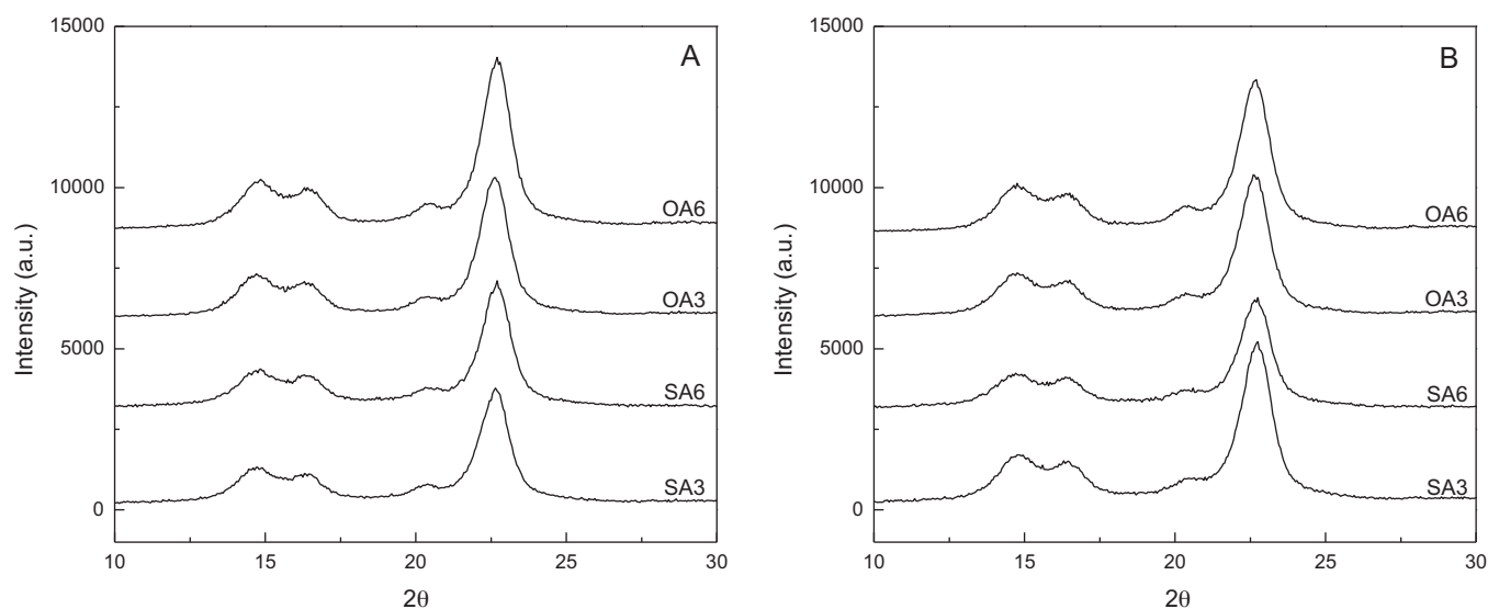
Fig. 5. X-ray diffractograms of selected solid samples after hydrolysis in (A) oven and (B) microwave.
