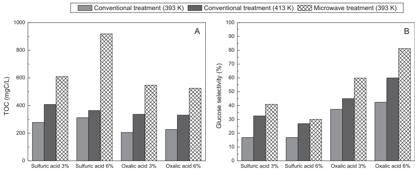
Fig. 4. (A) TOC values for cellulose hydrolysis in different hydrothermal conditions after 6 h of hydrolysis. (B) Glucose selectivity obtained from cellulose hydrolysis after 6 h.
