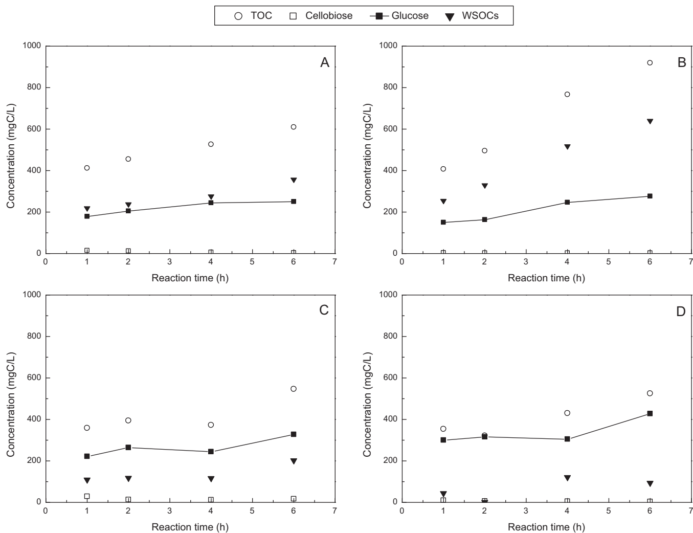
Fig. 3. Changes in aqueous product concentration (mg/L) versus reaction time during cellulose hydrolysis assisted by microwave irradiation at 393 K. Cellulose samples pretreated with (A) 3 wt.% of sulfuric acid (SA3), (B) 6 wt.% of sulfuric acid (SA6), (C) 3 wt.% of oxalic acid (OA3) and (D) 6 wt.% of oxalic acid (OA6).
